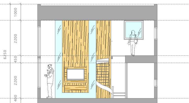
SECTION \frac{1}{50}
